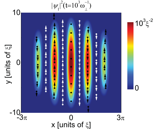
FIG. 10. (Color online) The density profile of \psi_1 at t = 10^3\omega_\perp^{-1} of the real-time dynamical evolution with the same parameters as Fig. 2. The initial value is chosen as the ground state in Fig. 2 plus a Gaussian noise of level 0.5%. The vortices of both the two components are marked by dots ( \bullet ), and arrows are added to show the direction and magnitude of the velocities of the vortex move.
