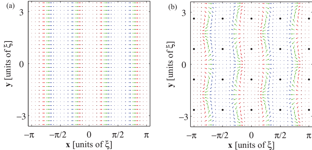
FIG. 4. (Color online) The vectorial representations of the pseudospin \mathbf{S} projected onto the x - y plane for (a) \Omega = 0 , T = \pi\xi , and (b) \Omega = 0.6\omega_{\perp} , T = \pi\xi . The colors ranging from blue to red describe the values of S_z from -1 to 1 . The locations of the vortices are marked by black dots ( \bullet ).
