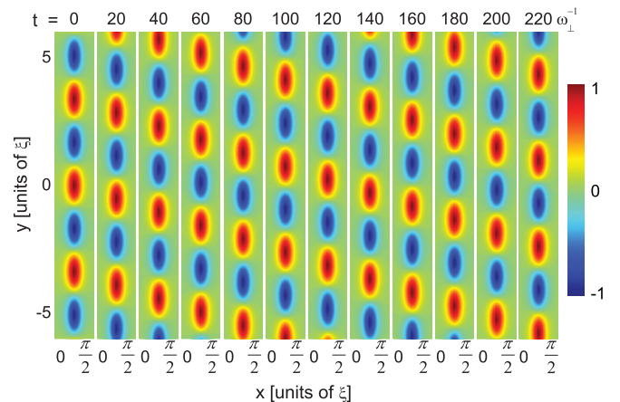
FIG. 11. (Color online) Time evolution of the pseudospin density S_x in a domain wall at the region of [0, \frac{\pi}{2}, -6, 6] in the presence of a Gaussian noise of level 0.5%. The numerical simulation process is the same as Fig. 10.
